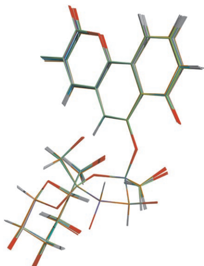
Figure 3. The 10 conformers of 2 ( RSSR configuration) with lowest energies found in floating chirality calculations (acetate moieties are not shown). The structures have been superimposed on the carbon atoms of the furanose ring. The average pairwise rmsd [17] is 0.106 Å.
